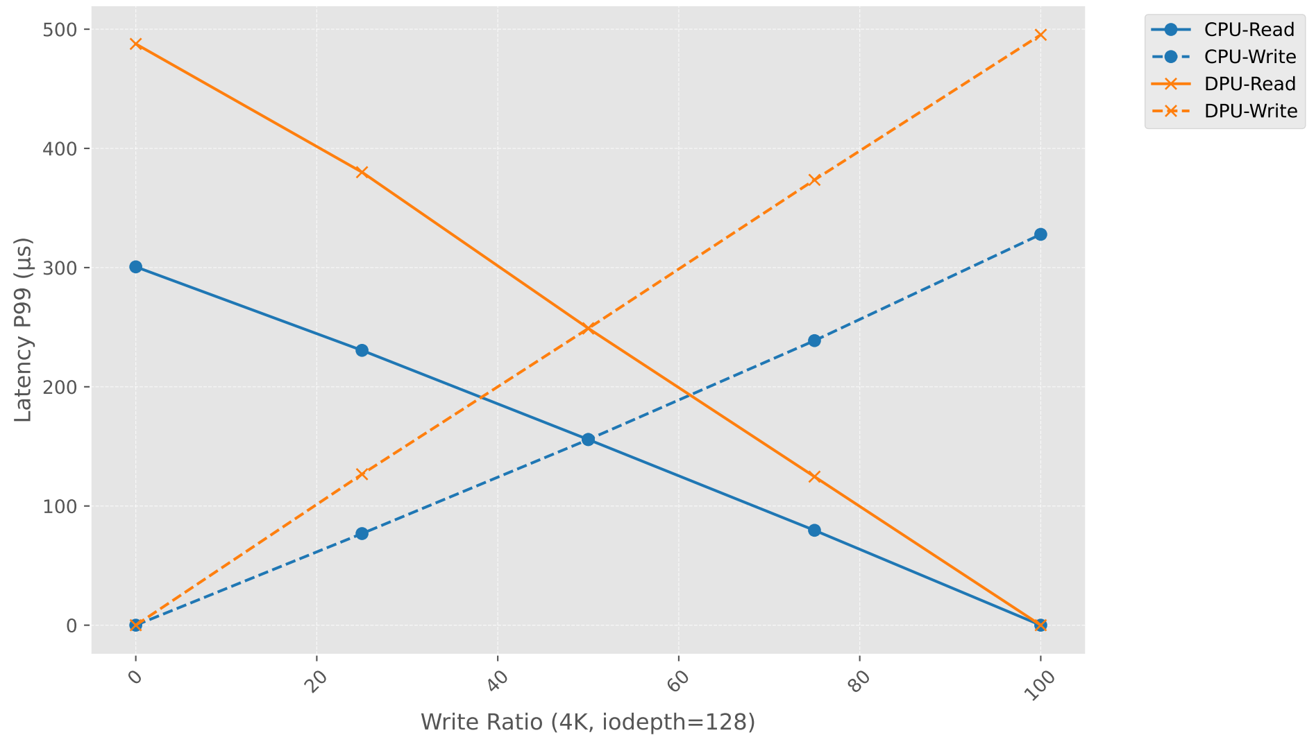
Latency P99 vs Write Ratio (4K, iodepth=128)
